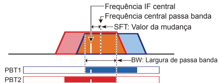
Tela FILTER (SSB) (ao operar o Twin-PBT)
